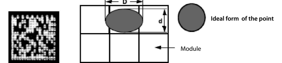
Figure 3.6.2-4 Elongation
